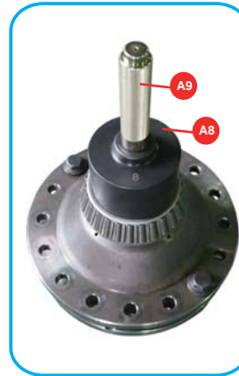
Install the differential front bearing: 安裝差速器前培林
