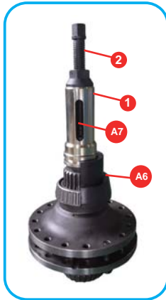
Remove the differential front bearing: 拆卸差速器前培林
