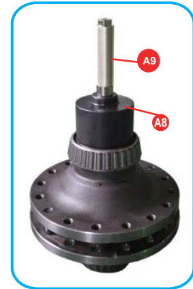
Install the differential rear bearing: 安裝差速器後培林
